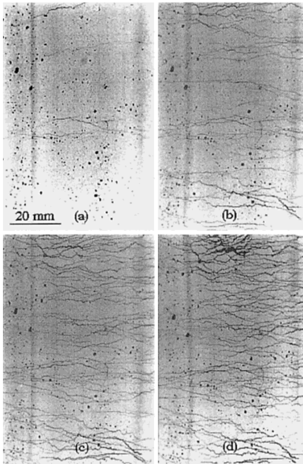
Figure 17 Damage evolution as a function of deformation on uniaxial tensile specimens (a) \epsilon = 0.3\% , (b) \epsilon = 2.2\% , (c) \epsilon = 4.2\% , and (d) “ \epsilon ” = 5.9%. 15
